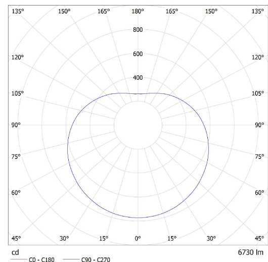
Lucis ZK.P3.500.X POLARIS ZK LED / LDC (Polar)
